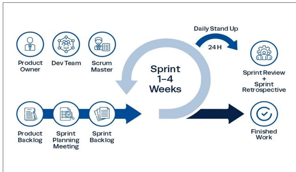
Figure 5 - Méthodologie Scrum [6]
